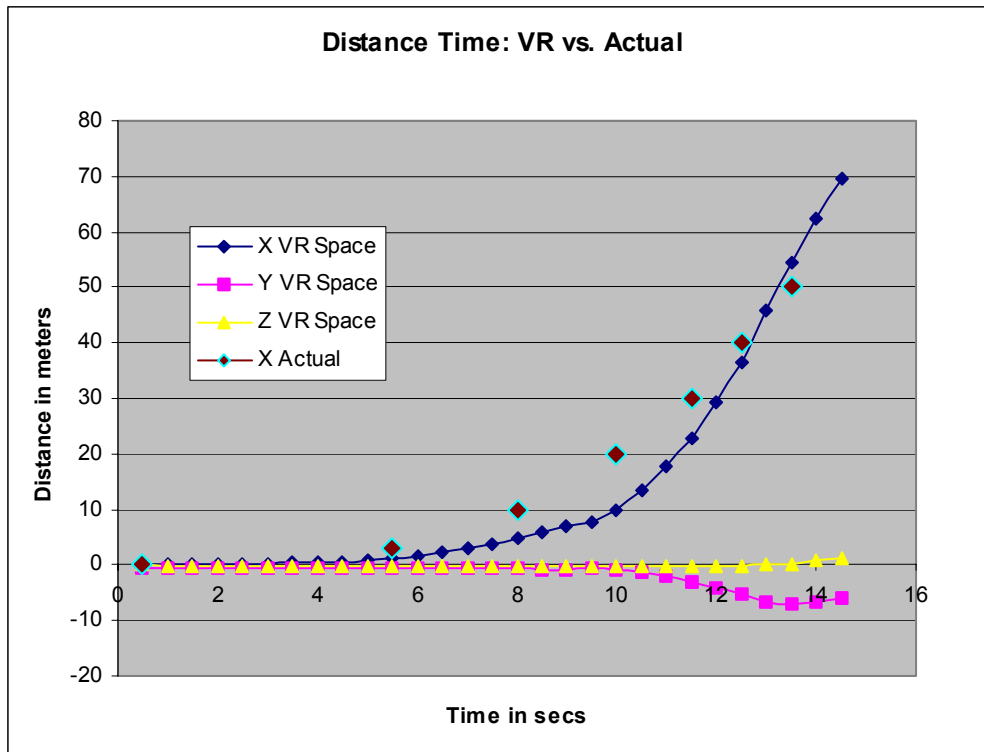
Figure 6. Comparison, Virtual and actual test sled.
