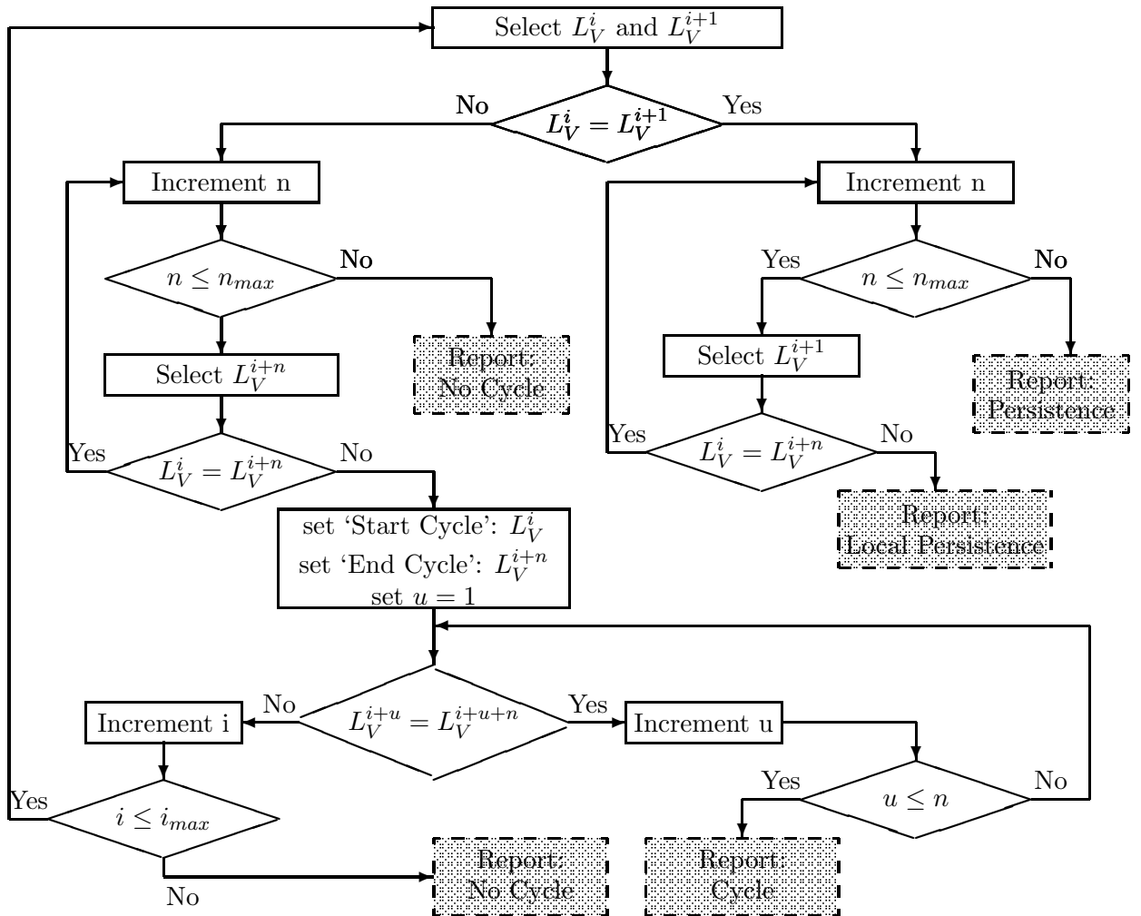
Figure 5.6: Repetition cycle detection algorithm.
